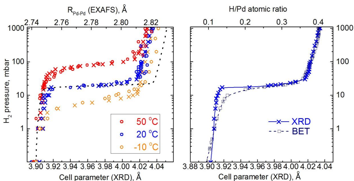
Figure 3. (left) Comparison of Pd-Pd interatomic distances obtained from EXAFS (circles) with cell parameter determined by XRD (crosses). Black dashed curved corresponds to the Pd black isotherm. (right) XRD measurements (crosses, blue line) vs volumetric data (squares, dashed navy line).
